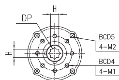
VALVE MOUNTING
