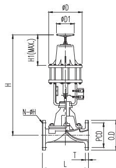
Single Acting
