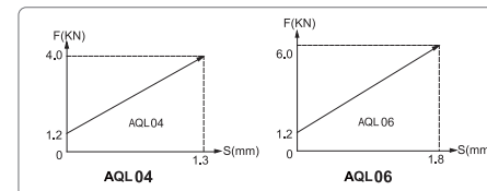
F : Closing(opening)force
